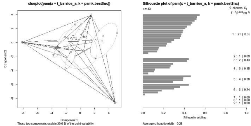
Fig. 3. PAM CLustering Results for Data Without Disallowed Repeated Check-ins
