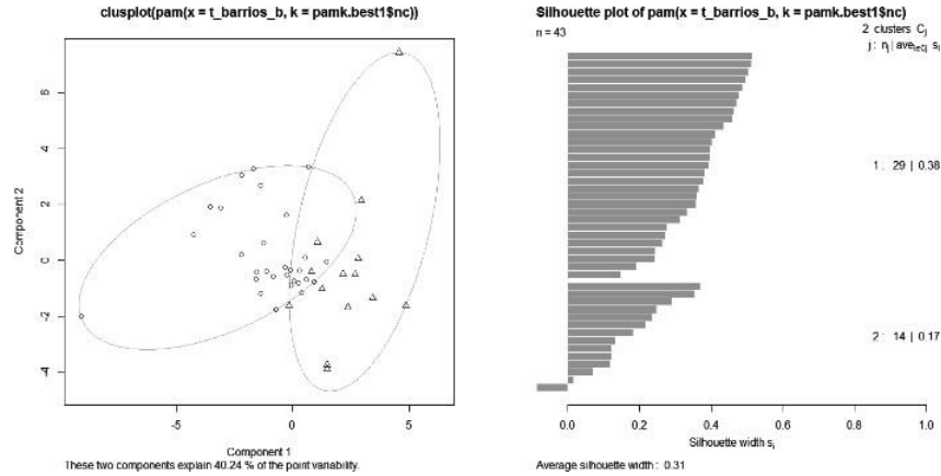
Fig. 2. PAM Clustering Results for the dataset before the disallowed check-ins were removed.
