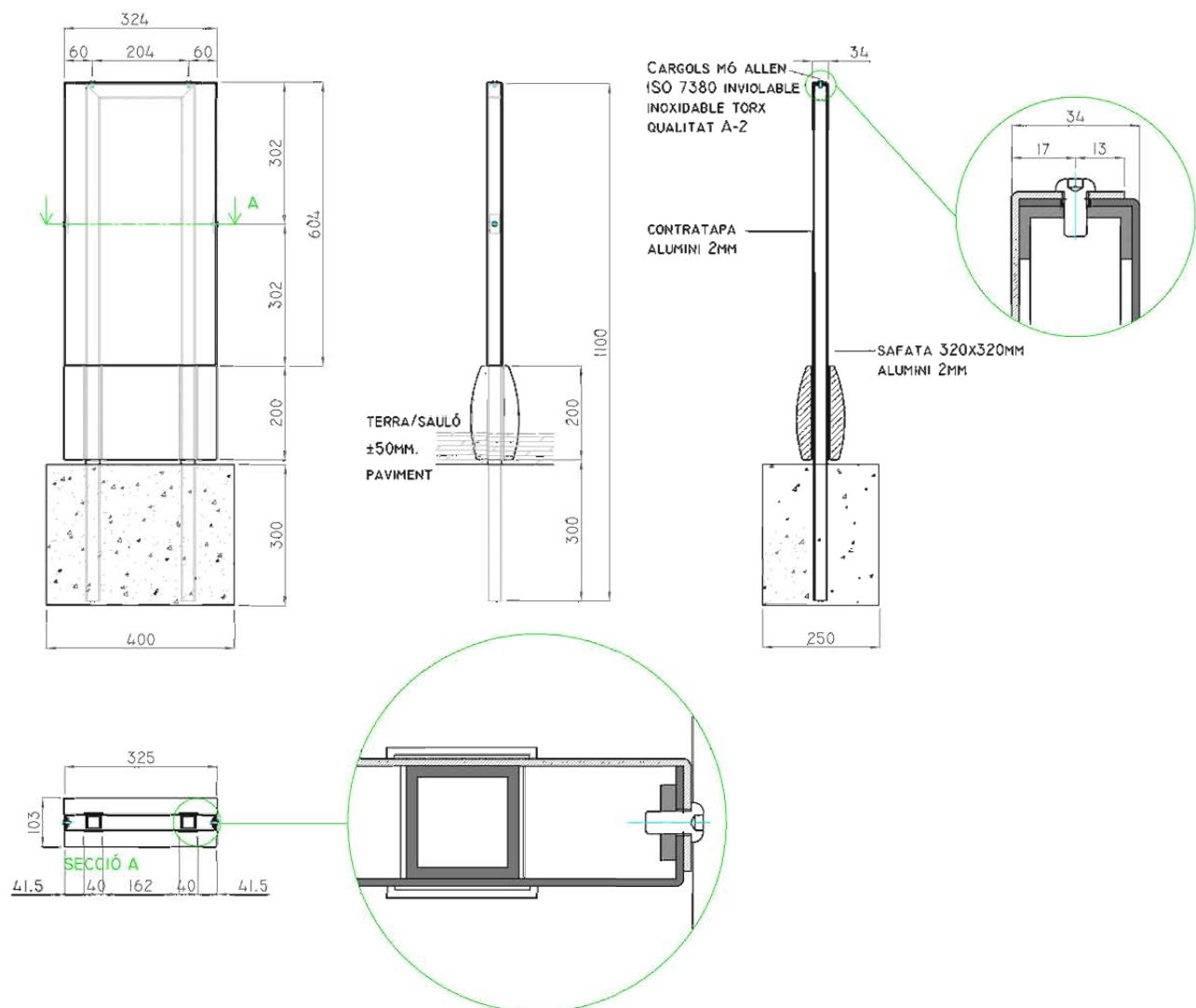
CONTRATAPA ALUMINI
