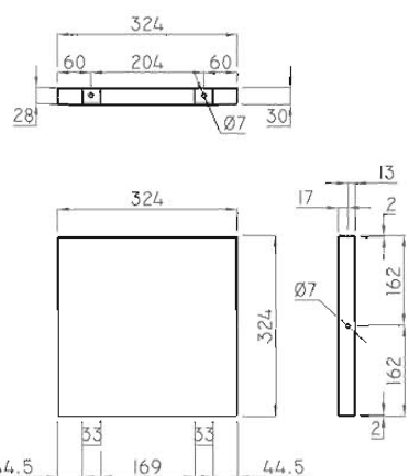
CONTRATAPA ALUMINI
