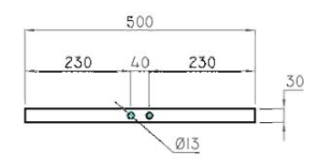
TUB PER A TRANSPORT
