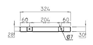
CONTRATAPA ALUMINI
